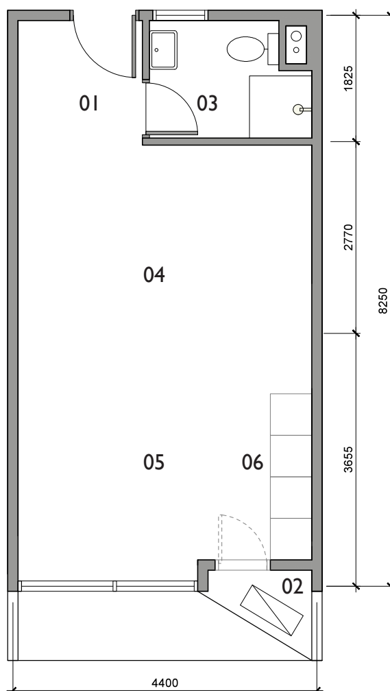
Type A1 403 sq.ft (37.5 sq.m)
