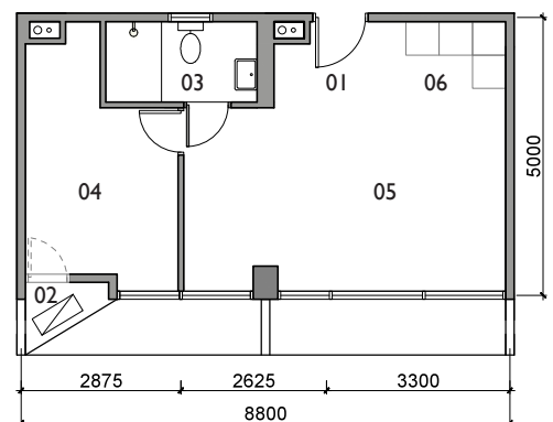
Type B2 490 sq.ft (45.5 sq.m)
