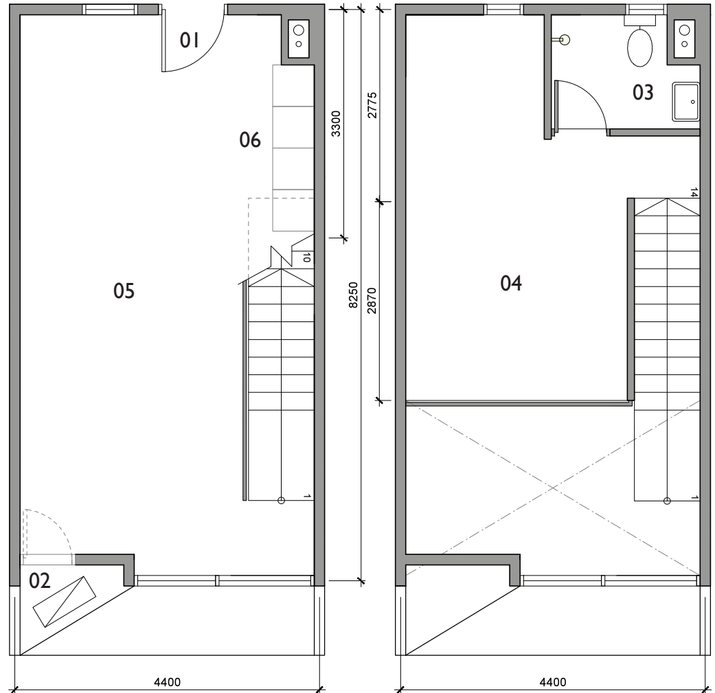
Type A1 669 sq.ft (62 sq.m)
