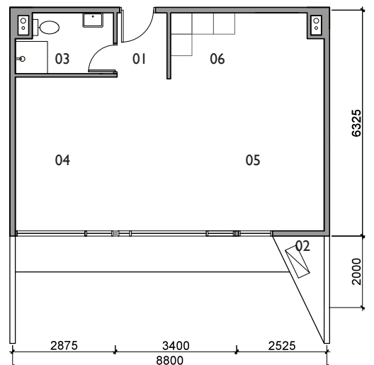
Type D2 620 sq.ft (58 sq.m)
